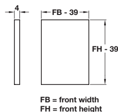
Glass dimensions
