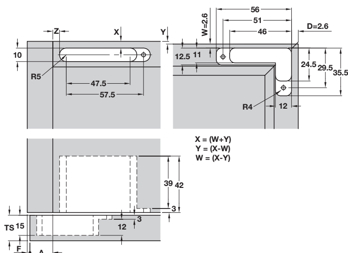
Installation dimensions
