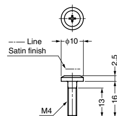
⑤ Truss head screw M4×16
