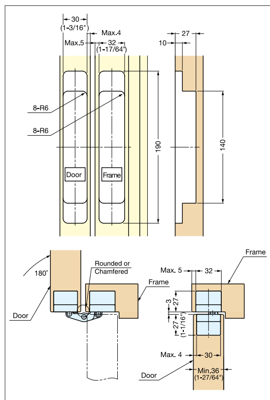
Bore Dimensions
